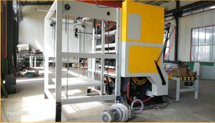
feeder unit
